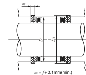
m = f + 0.1mm (min.)
