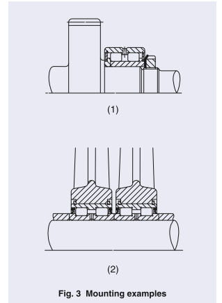
Fig. 3 Mounting examples
