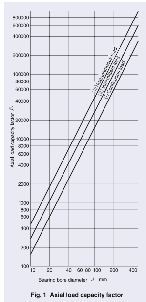
Fig. 1 Axial load capacity factor
