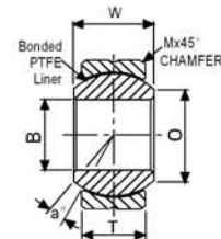
SCOM..T
