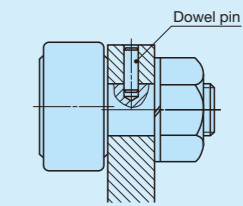
Fig. 8 Mounting examples of Solid Eccentric Stud Type Cam Followers
