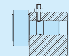
Fig. 10 Mounting examples of Easy Mounting Type Cam Followers
