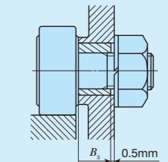
Fig. 9 Length of mounting hole for Eccentric Type Cam Followers
