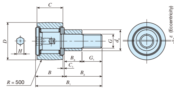
CFE...VBR Outside diameter of eccentric collar d_e 9 to 13 mm (1)
